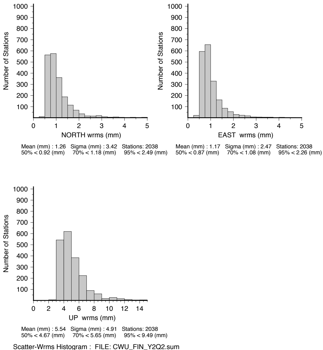
Figure 1: CWU solution histograms of the North, East and Up RMS scatters of the position residuals for 2038 stations analyzed between December 15, 2020 and March 21, 2020. Linear trends and annual signals were estimated from the time series.
