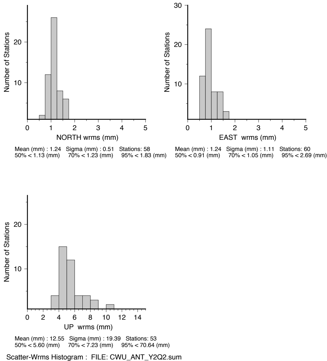
Figure A.1: CWU solution histograms of the North, East and Up RMS scatters of the position residuals for 60 stations in Antarctica analyzed between December 15, 2020 and March 21, 2020. Linear trends and annual signals were estimated from the time series.
